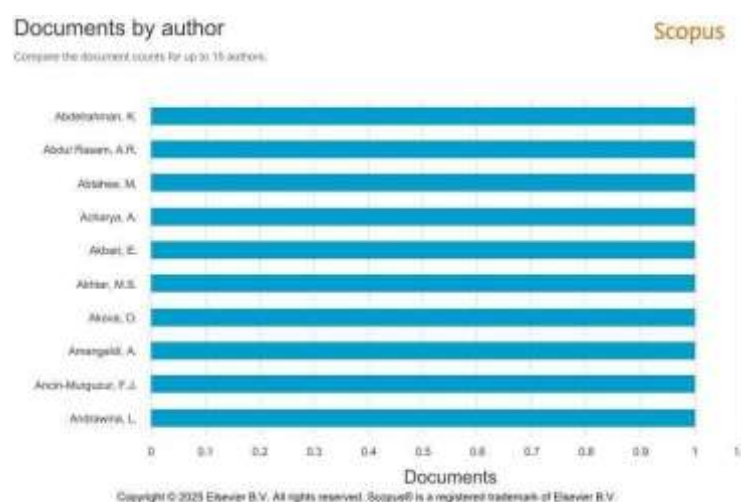
Gambar 1. Author Scopus
